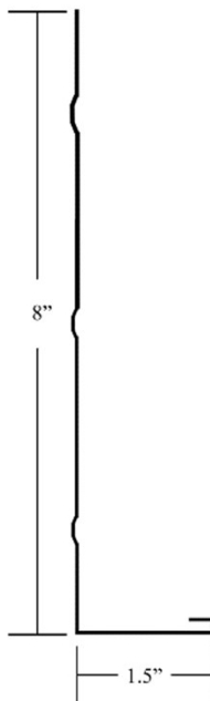
# 611 RF 8" F.C. 10" Girth.
