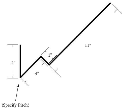
● # 507 Dam 20" Girth.
