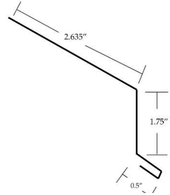
● #104 Eave 5.052" Girth
