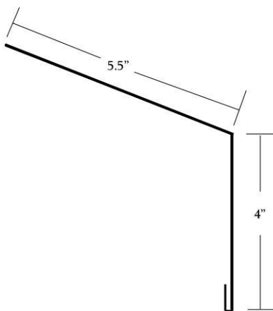
● #303 Flush Gambrel 10" Girth
