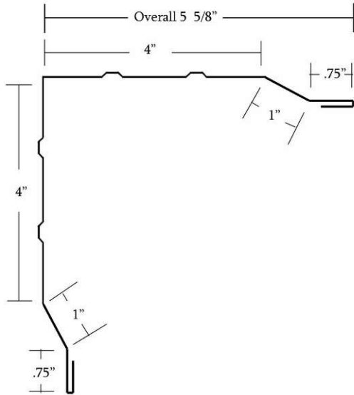
● #603 RF 4x4 Corner 12.25" Girth
