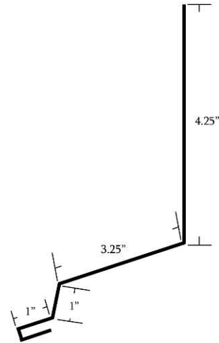
● # 402 Head Wall. 10" Girth.
