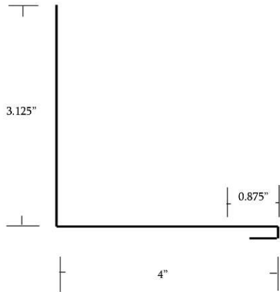
● # 408 Reg S.Seam Headwall 10" Girth.
