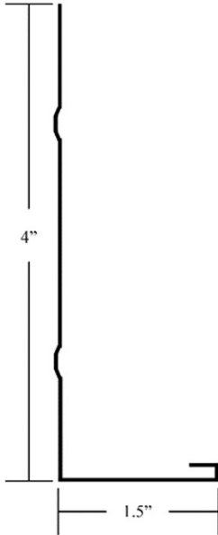
# 609 RF 4" F.C. 6" Girth.
