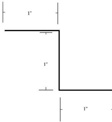
● #606 RF Step Z 4.50" Girth
