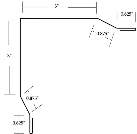
● # 701. 3X3 Corner 10" Girth.
