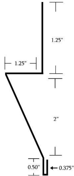
● # 003 Tall Rat Guard 5.5" Girth
