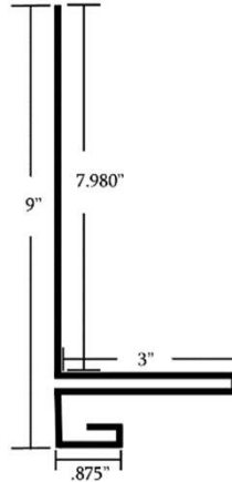
● #009 Garage Door Trim 14.625" Girth w/ 8" leg
