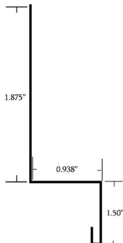
● #606 RF Step Z 4.50" Girth
