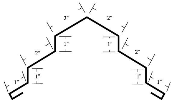
● # 304 Double Drop Ridge 15" Girth.
