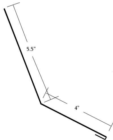
● #303-B Reverse Gambrel 10" Girth
