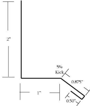
● #006 Stone Drip 4.375" Girth.
