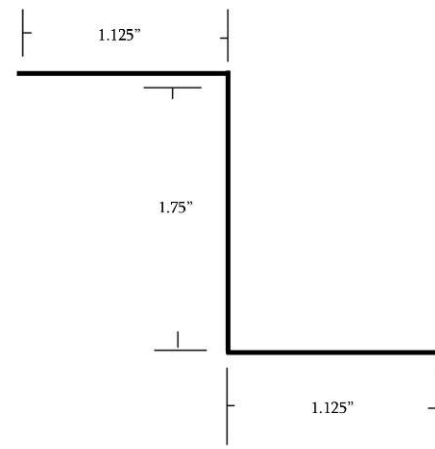
● # 909 Solid 1.75" Z 4" Girth
