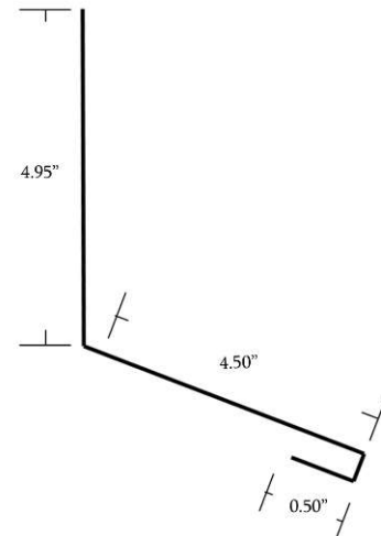
● # 405. Flush Head. 10" Girth.
