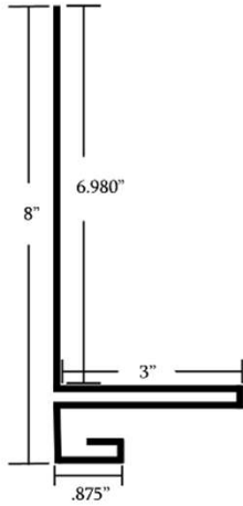
● #004 Garage Door Trim 13.625" Girth w/ 7" leg
