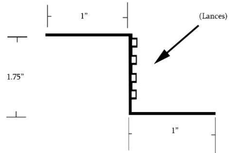
● # 909 Solid 1.75" Z 4" Girth
