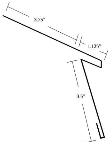
● #105 Eave 4" Face Drip 10" Girth
