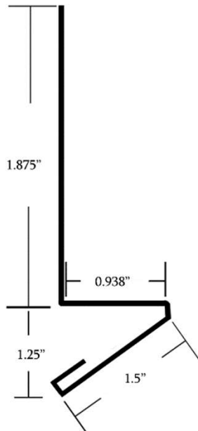
# 607 RF Rat Guard 4.5" Girth.
