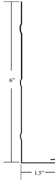
# 610 RF 6" F.C. 8" Girth.
