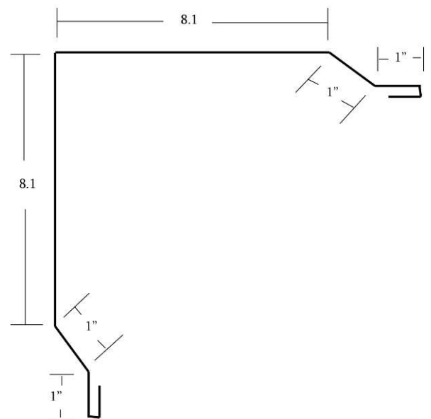
● # 704 Jumbo Corner 21.5" Girth.
